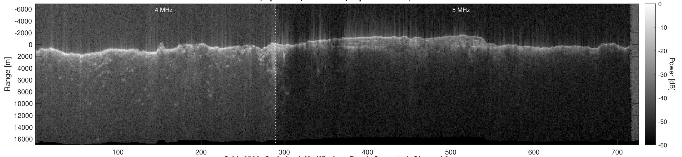
Orbit 6599, Optimized, No Window, Depth-Corrected, Channel 2
