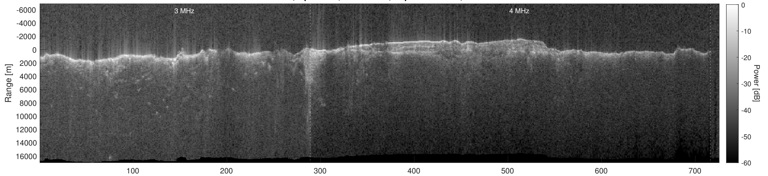
Orbit 6599, Depth-Corrected Cluttergram
