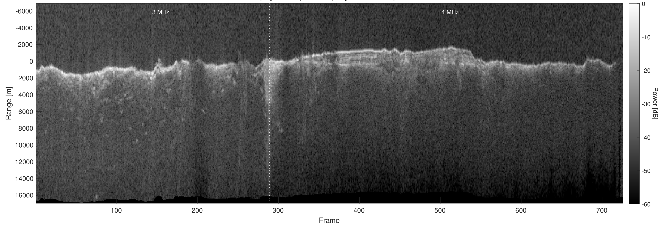
Orbit 6599, Optimized, Window, Depth-Corrected, Channel 2
