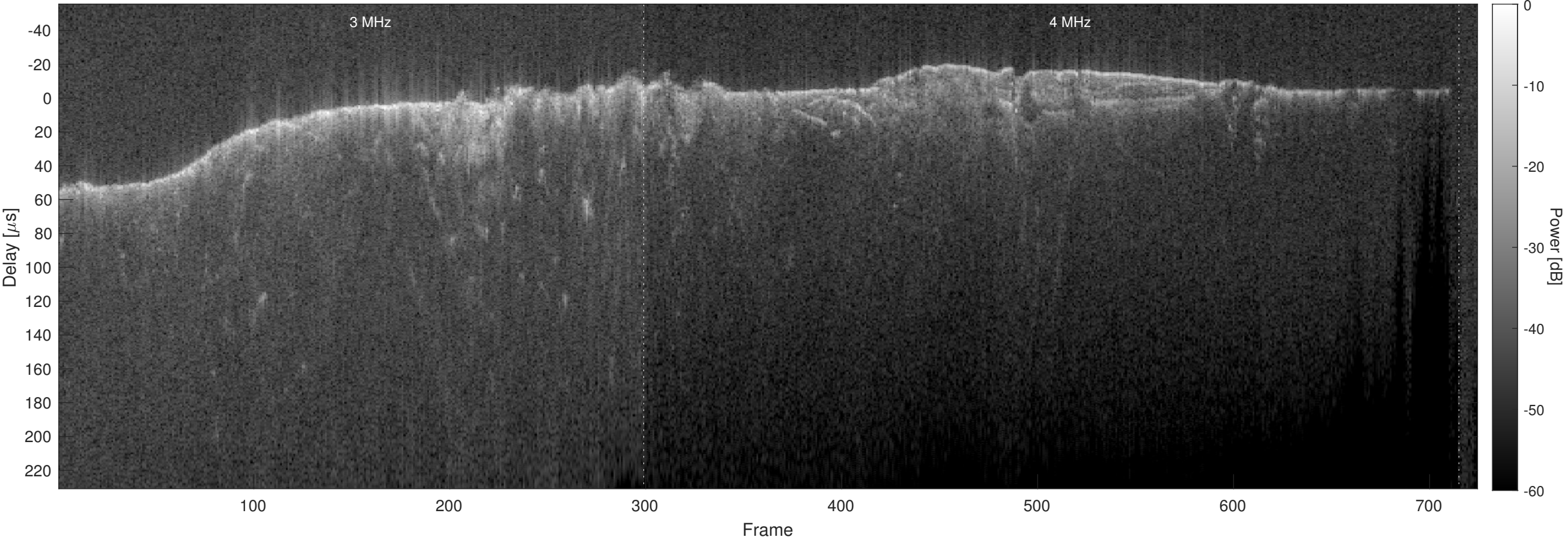
Orbit 6600, Optimized, No Window, Channel 2
