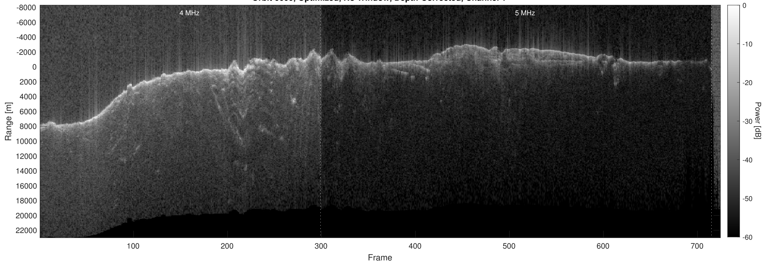
Orbit 6600, Optimized, No Window, Depth-Corrected, Channel 2
