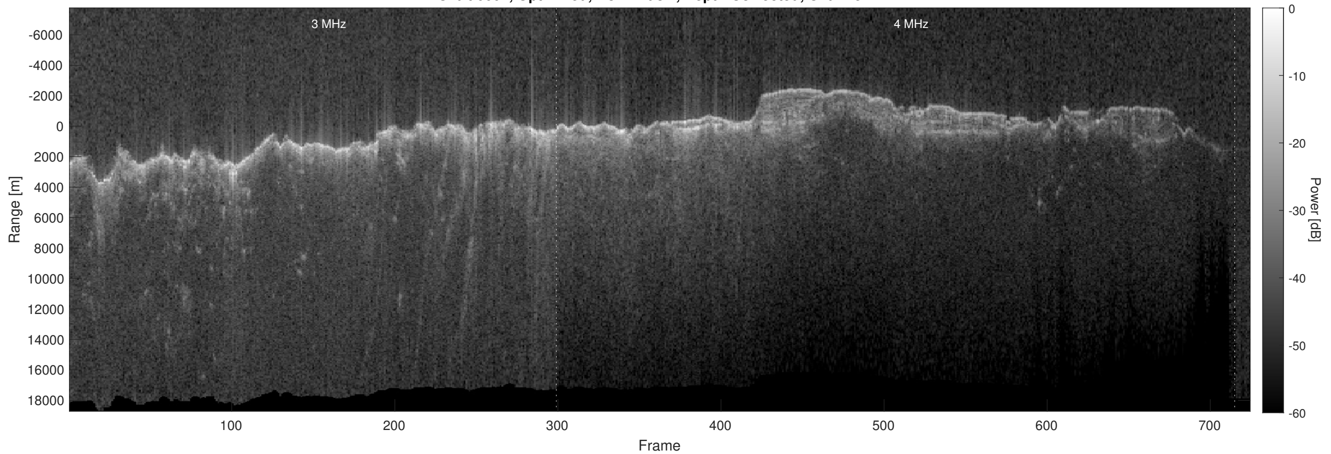
Orbit 6601, Optimized, No Window, Depth-Corrected, Channel 2
