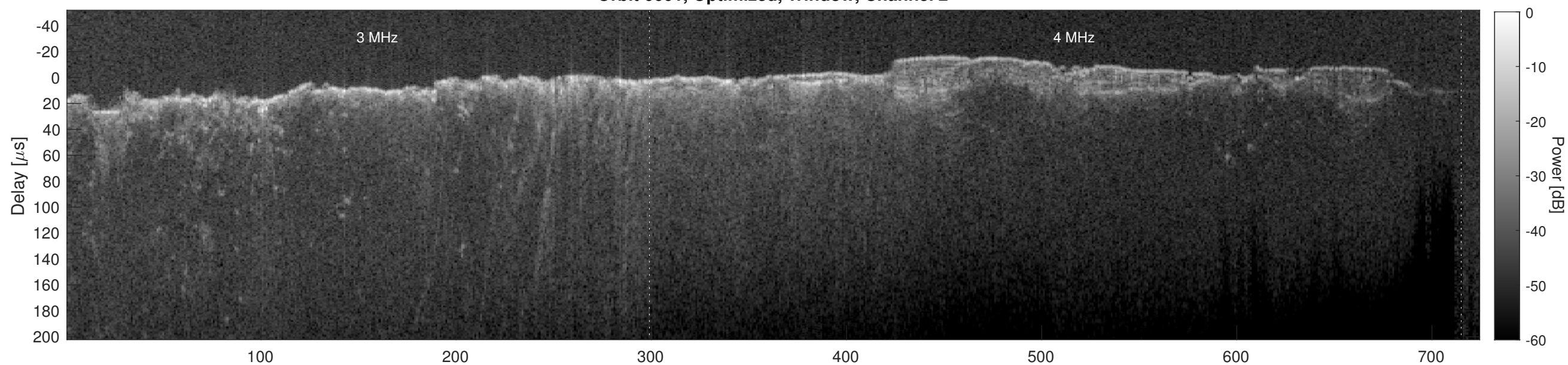
Orbit 6601, Cluttergram
