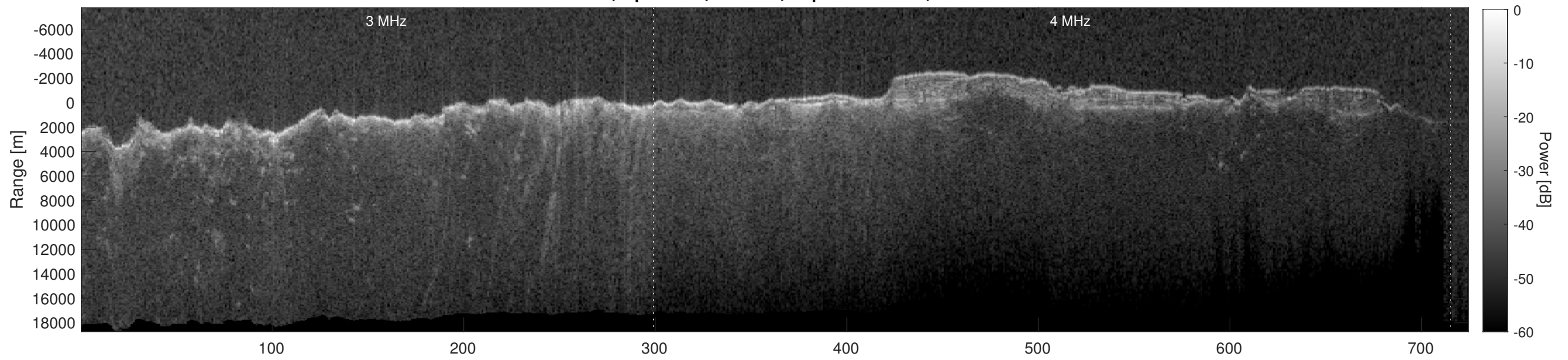
Orbit 6601, Depth-Corrected Cluttergram
