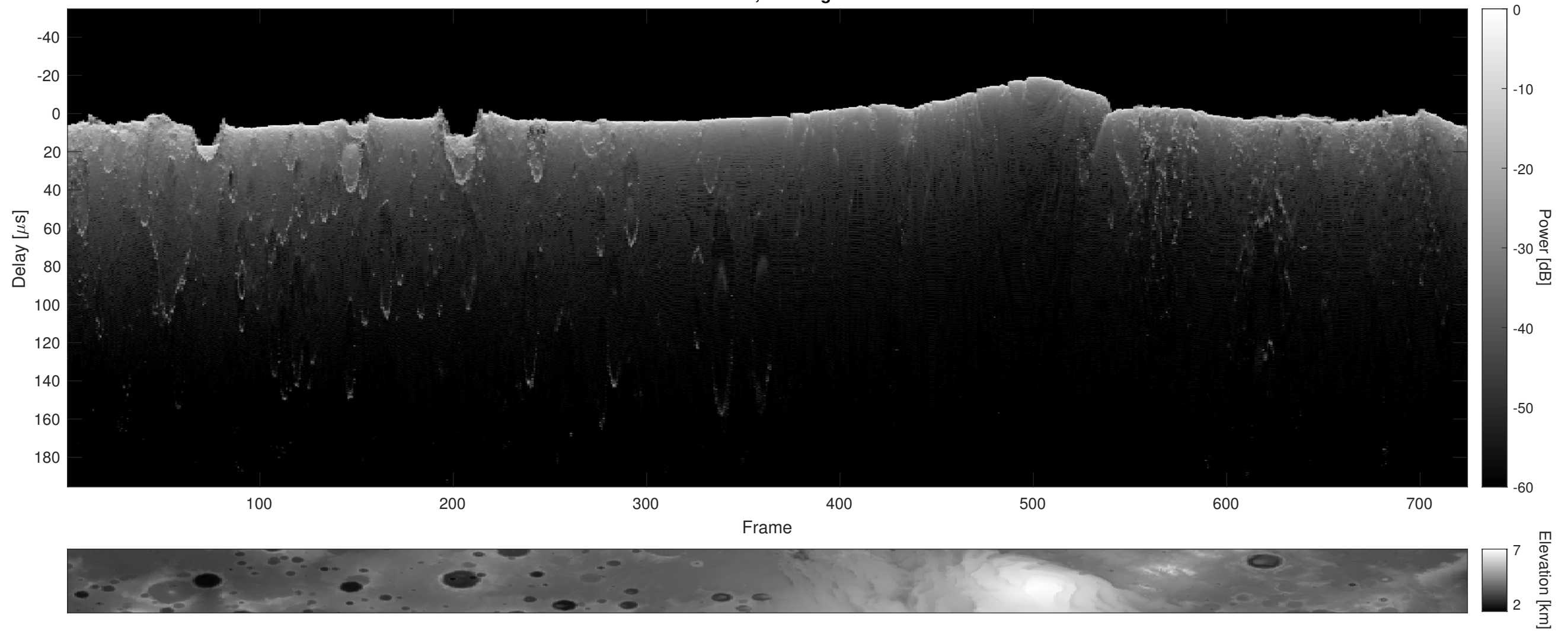
Orbit 6602, Cluttergram
