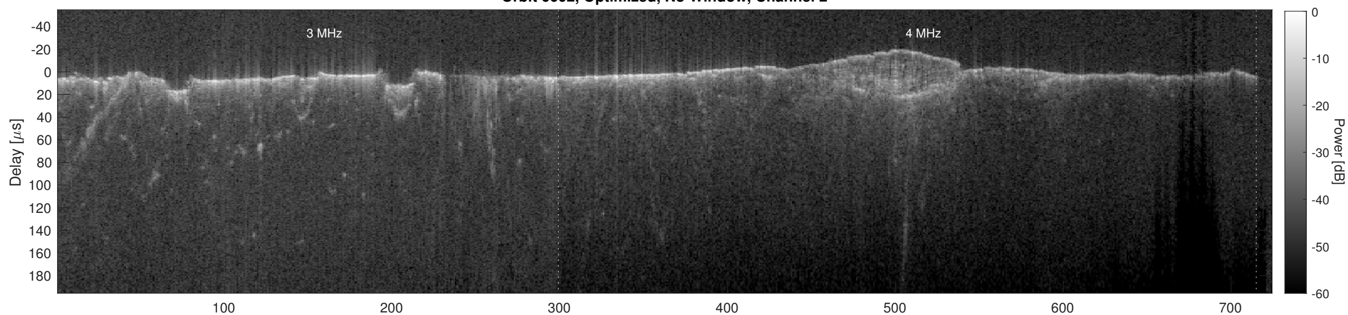
Orbit 6602, Cluttergram
