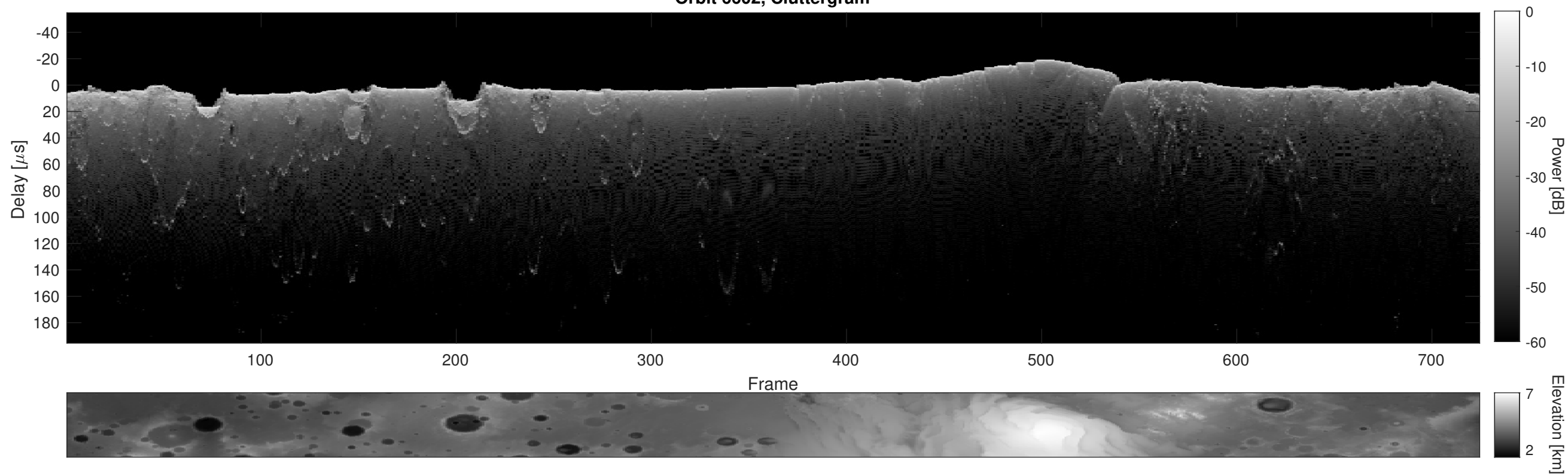
Orbit 6602, Cluttergram
