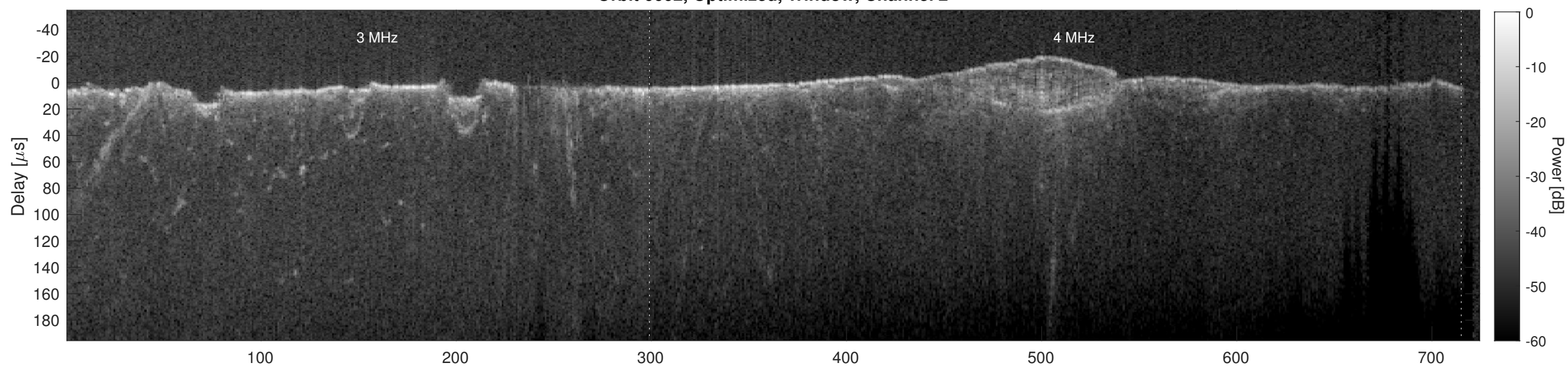
Orbit 6602, Cluttergram
