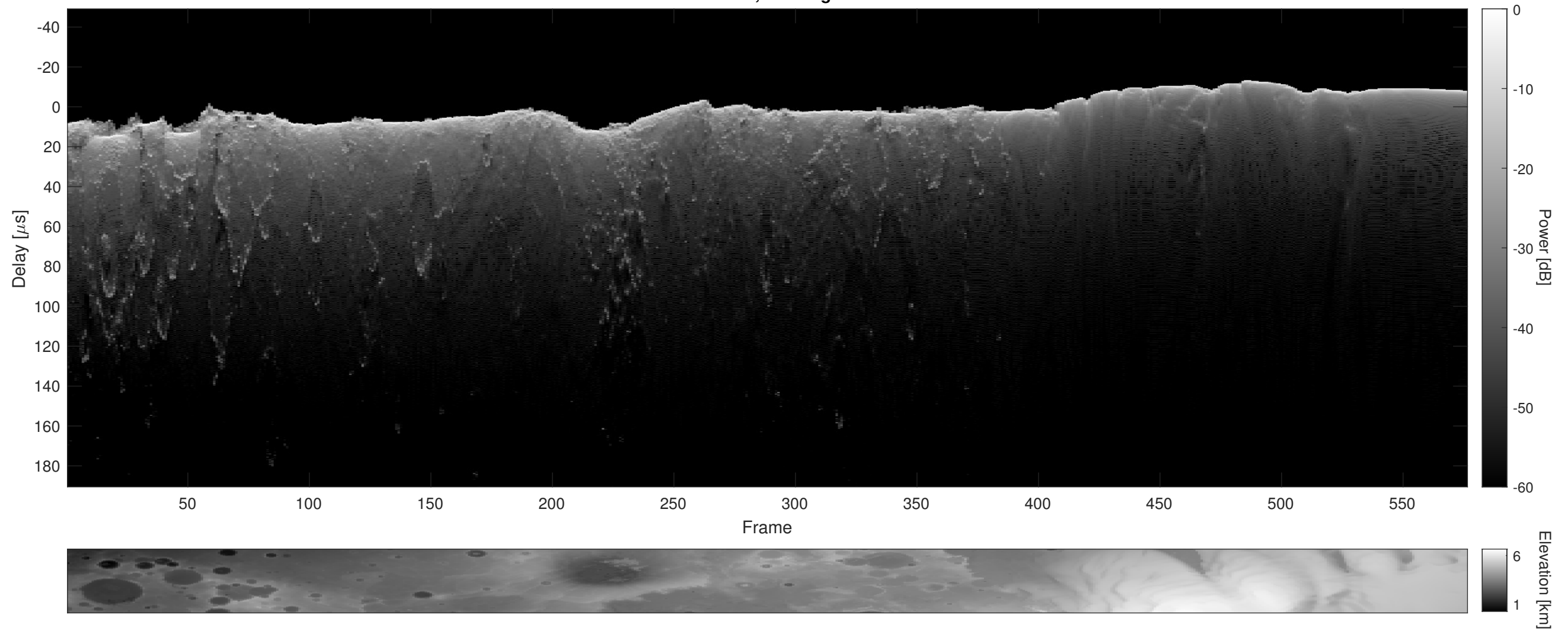
Orbit 6604, Cluttergram
