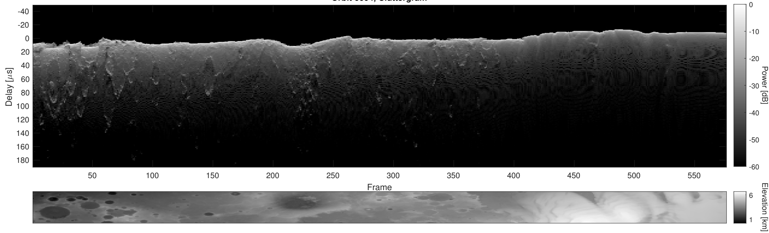
Orbit 6604, Cluttergram
