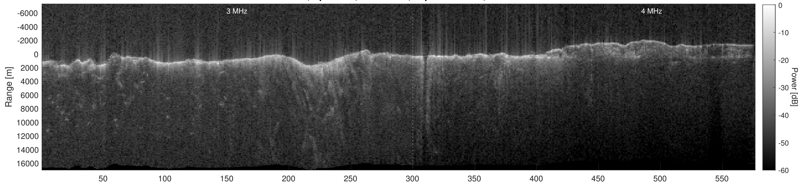
Orbit 6604, Depth-Corrected Cluttergram
