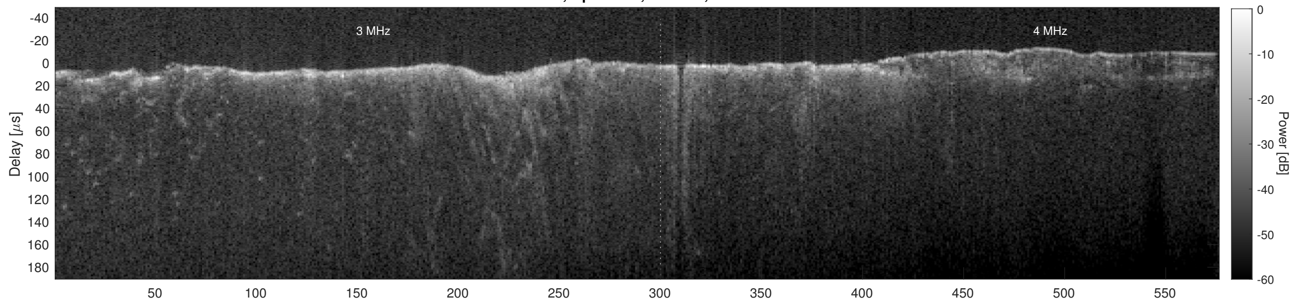
Orbit 6604, Cluttergram
