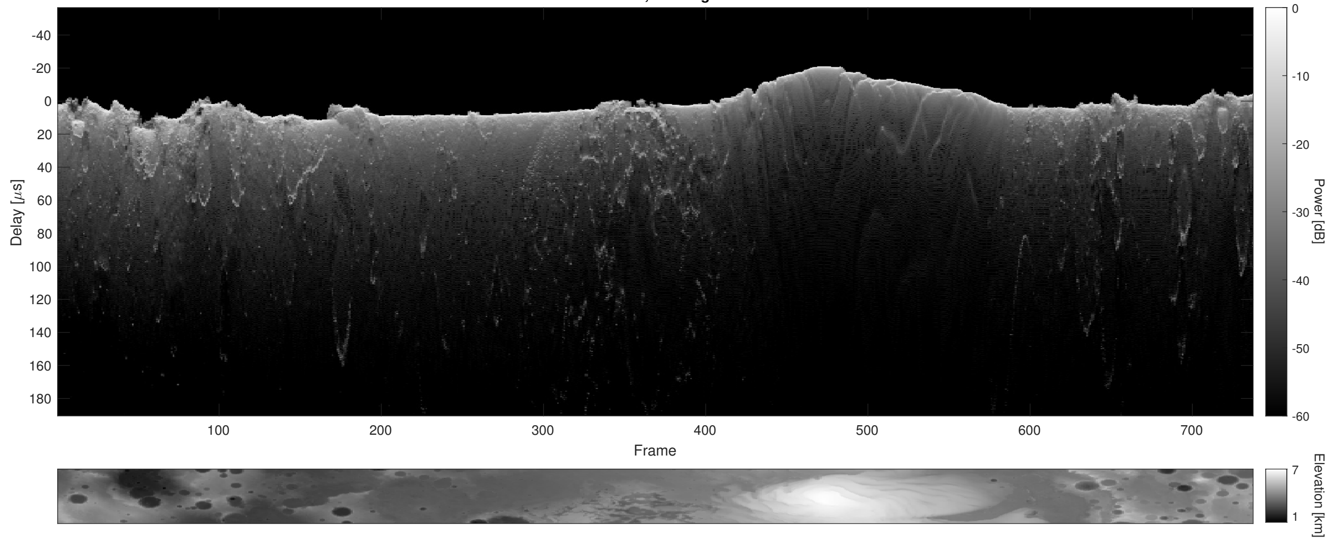
Orbit 6605, Cluttergram
