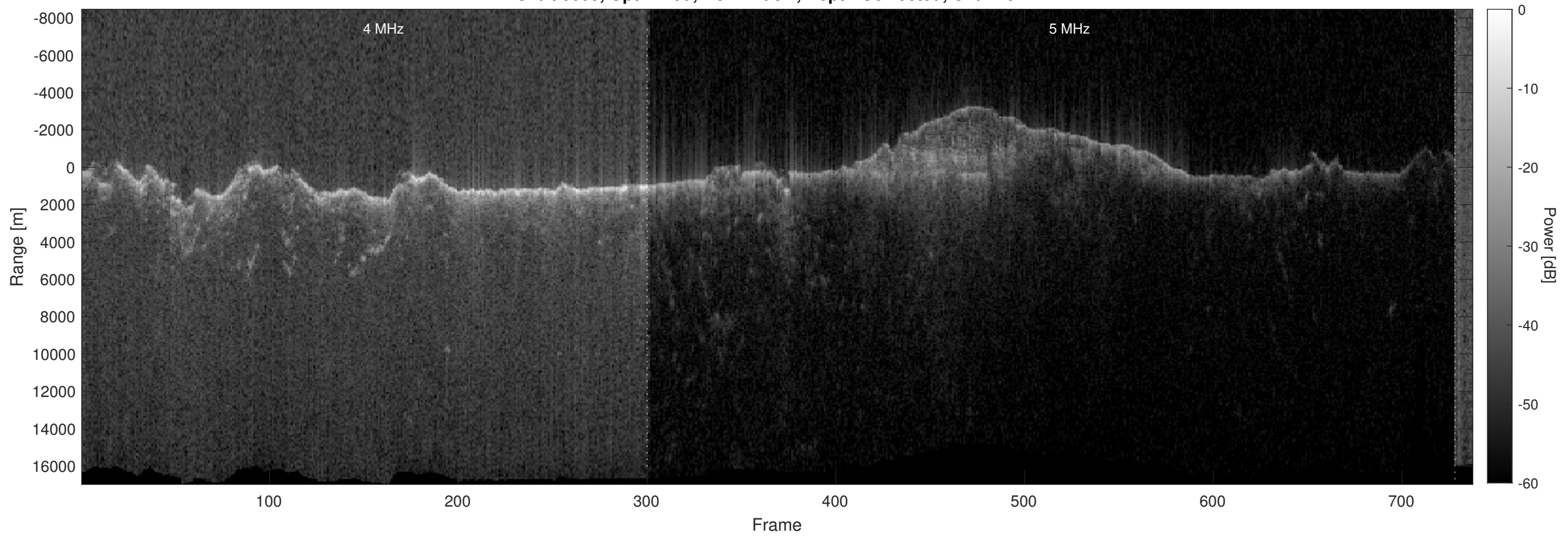
Orbit 6605, Optimized, No Window, Depth-Corrected, Channel 2
