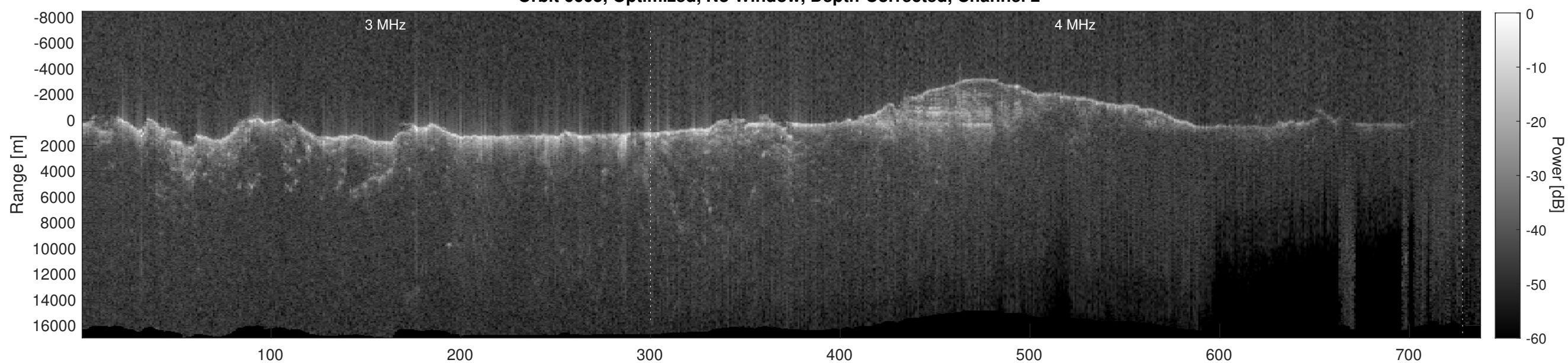
Orbit 6605, Depth-Corrected Cluttergram
