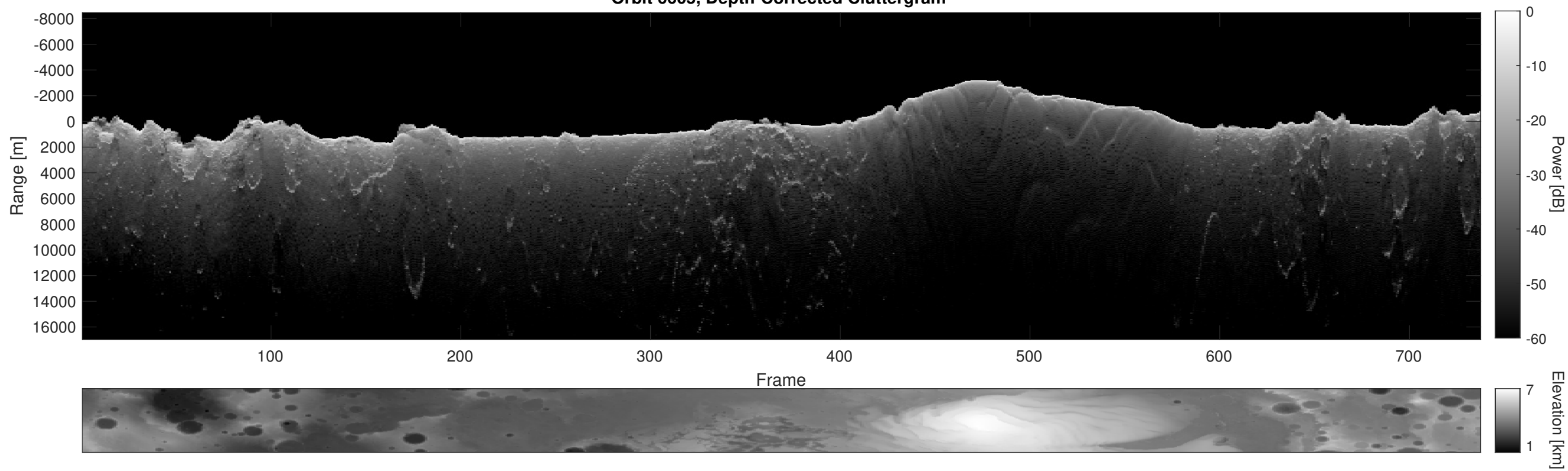
Orbit 6605, Depth-Corrected Cluttergram
