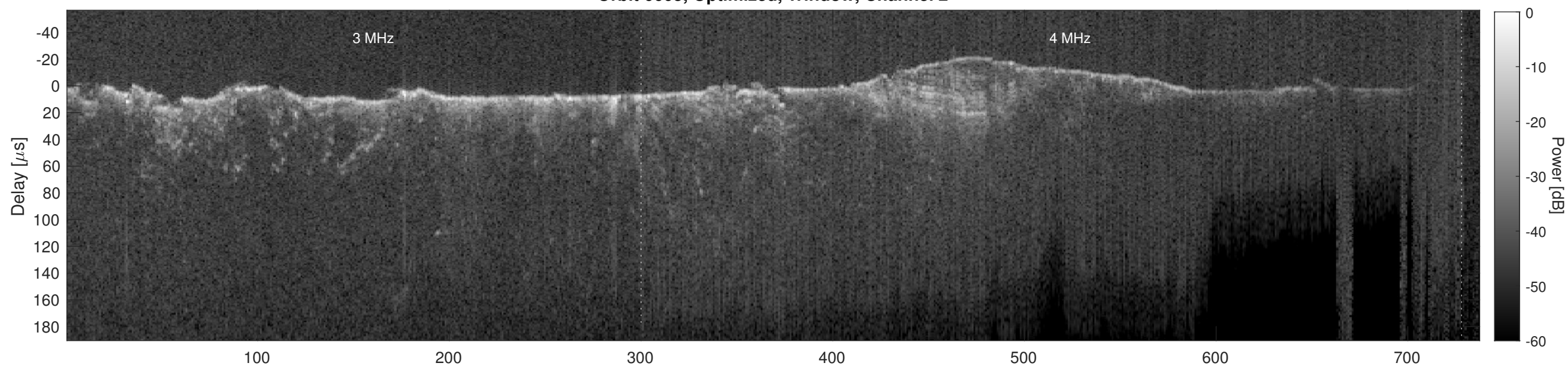
Orbit 6605, Cluttergram
