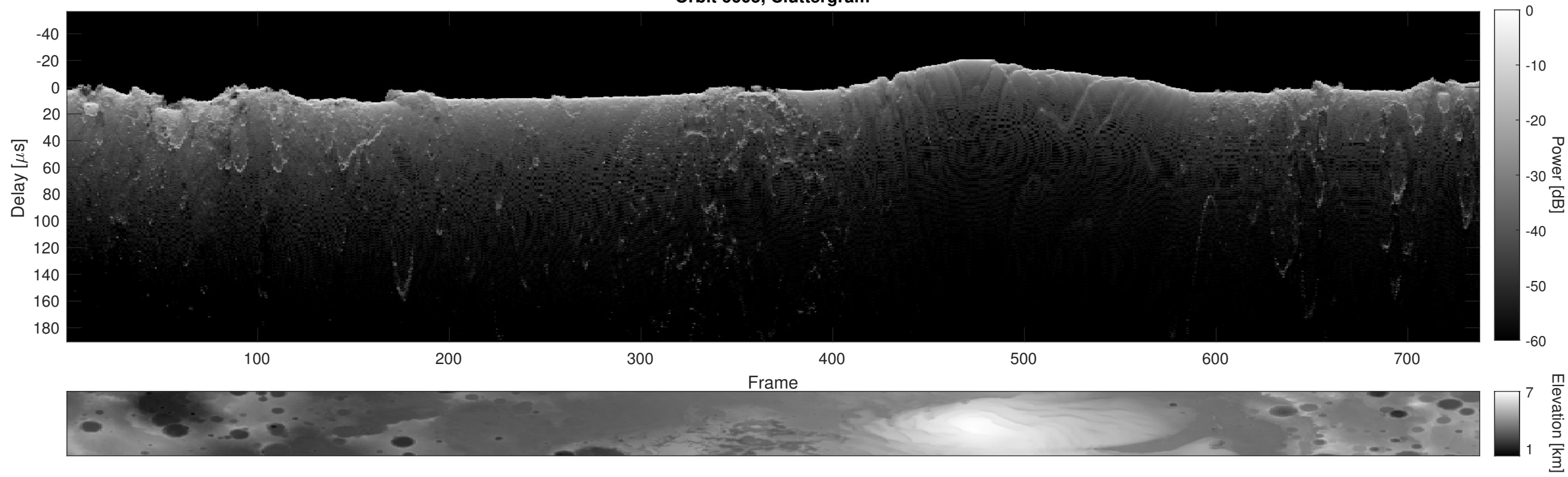
Orbit 6605, Cluttergram
