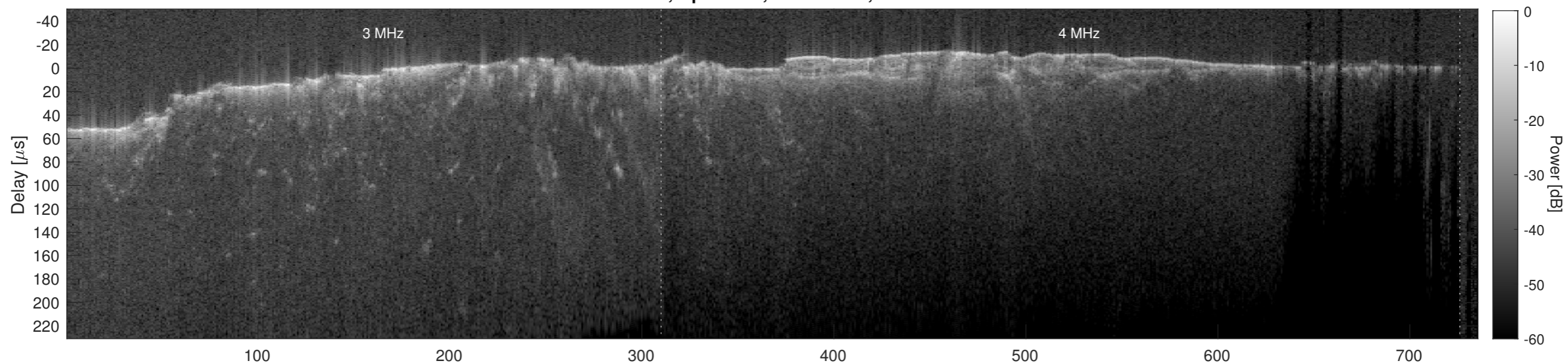
Orbit 6607, Cluttergram
