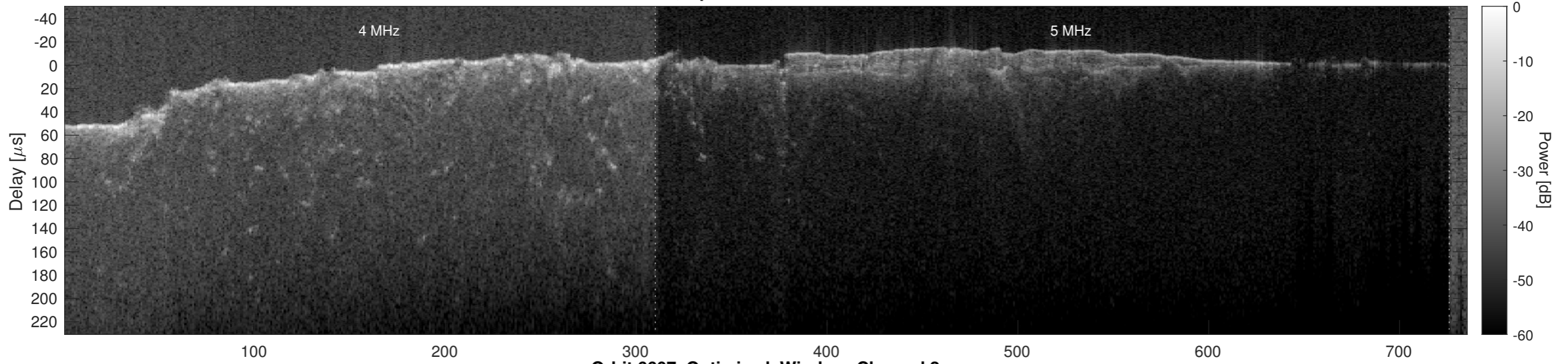
Orbit 6607, Optimized, Window, Channel 2
