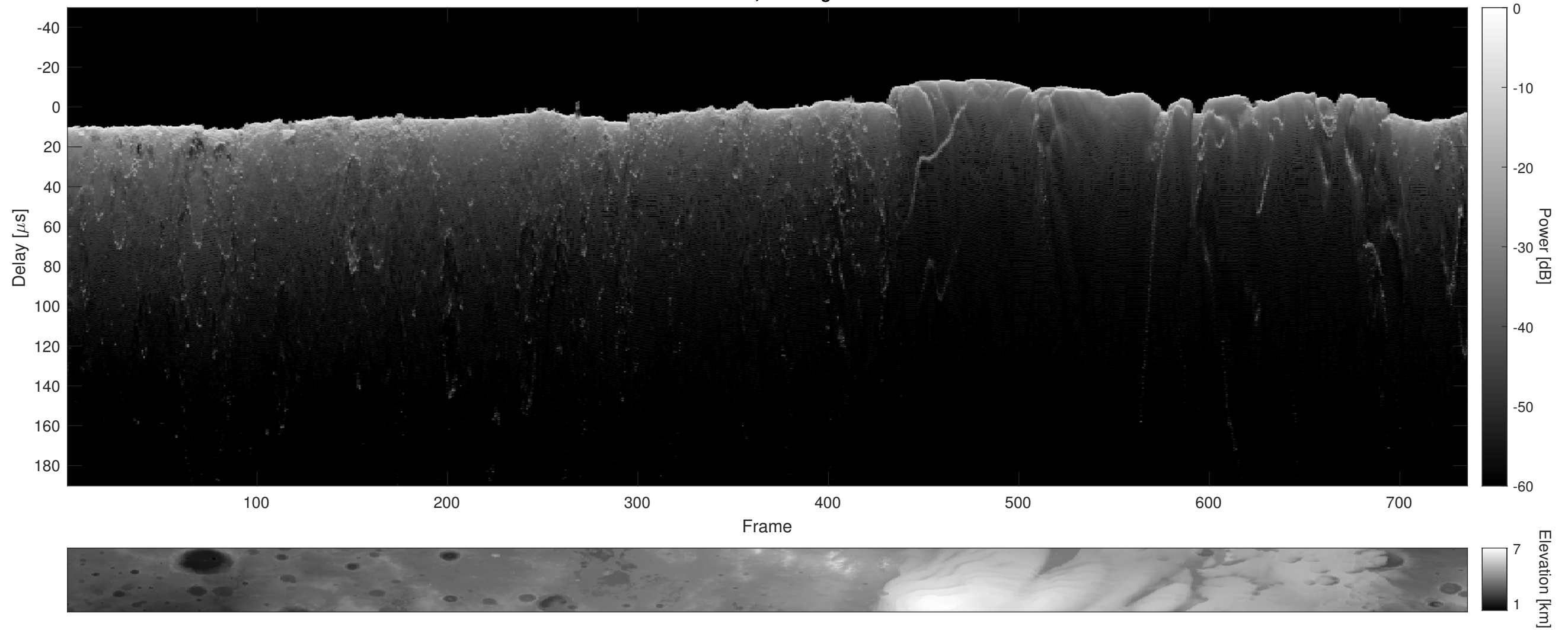
Orbit 6608, Cluttergram
