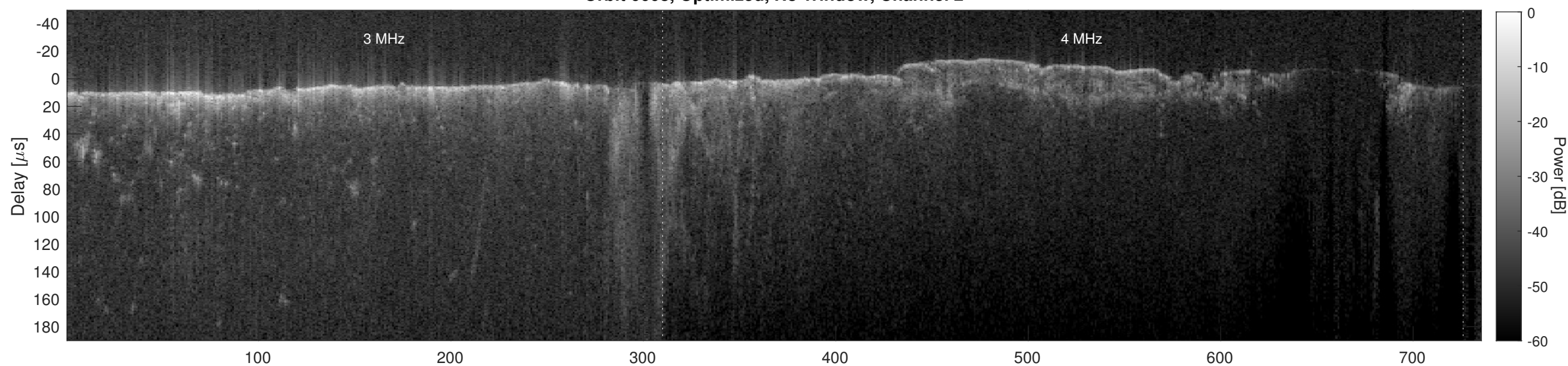
Orbit 6608, Cluttergram
