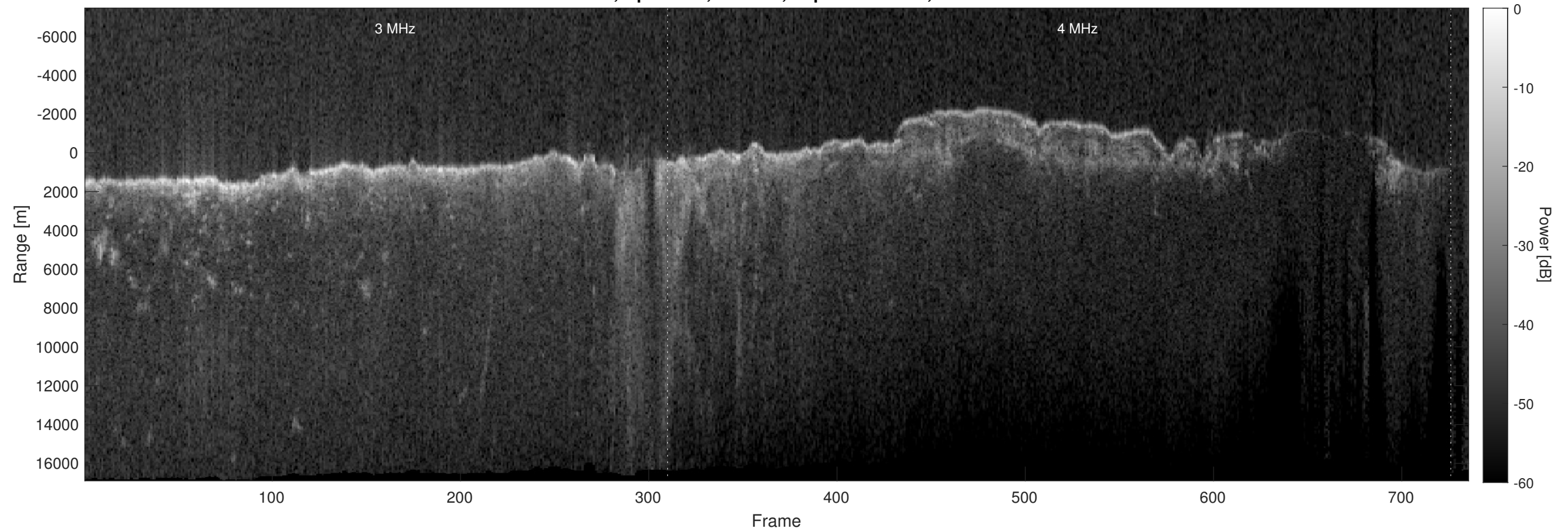
Orbit 6608, Optimized, Window, Depth-Corrected, Channel 2
