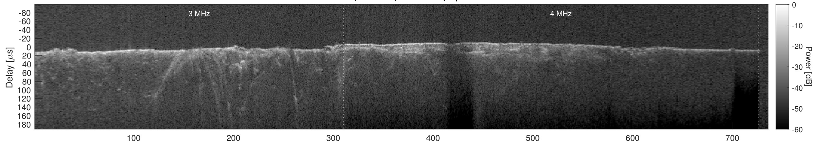
Orbit 6610, Cluttergram
