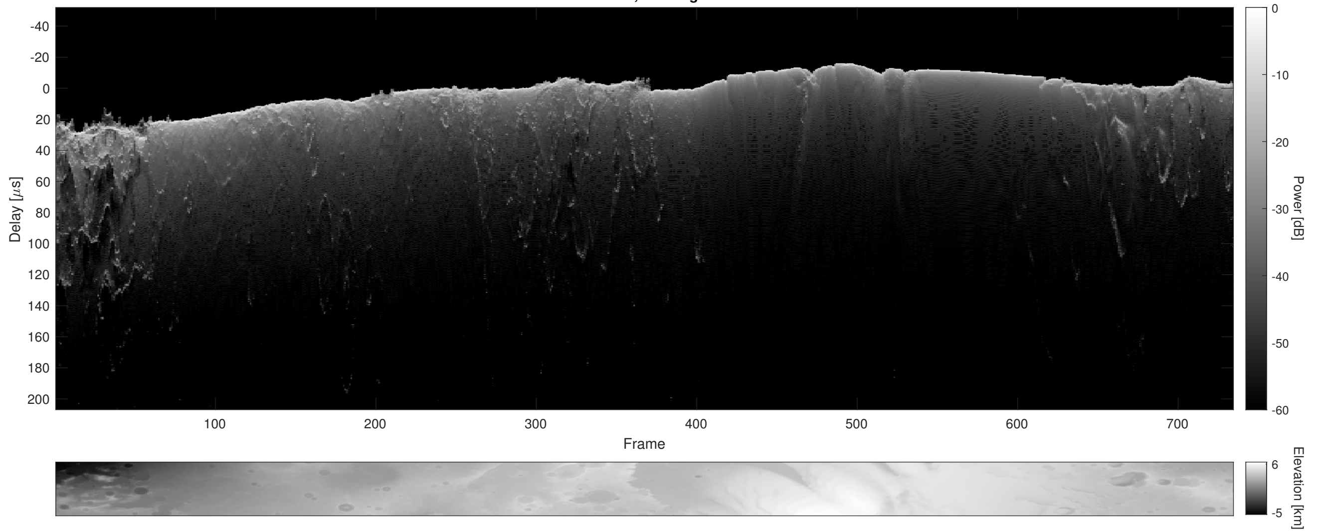
Orbit 6611, Cluttergram
