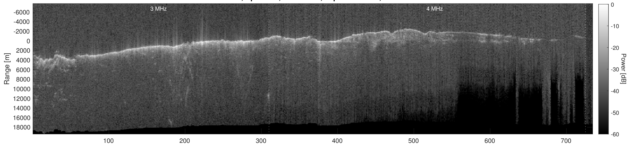
Orbit 6611, Depth-Corrected Cluttergram
