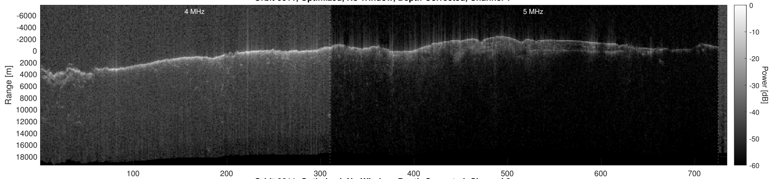
Orbit 6611, Optimized, No Window, Depth-Corrected, Channel 2
