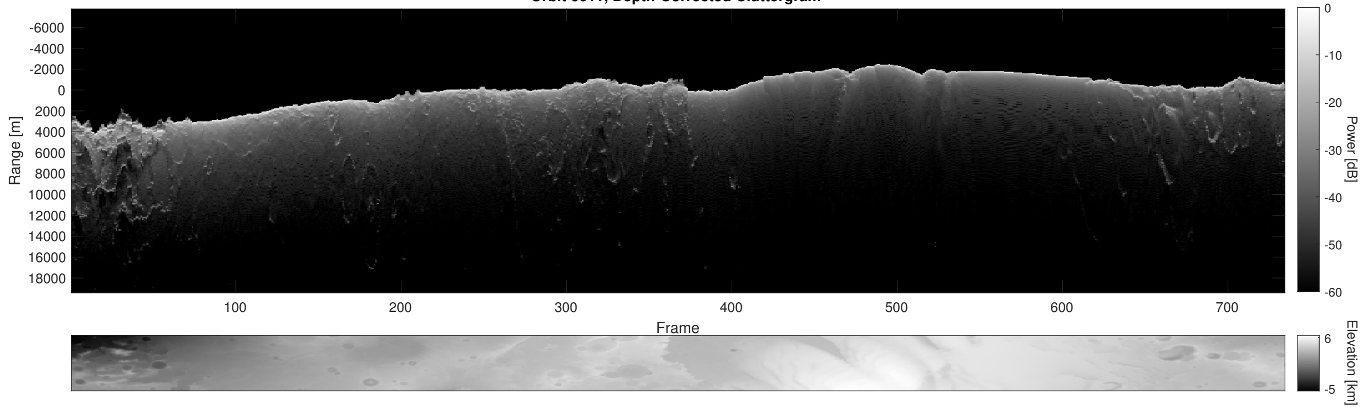
Orbit 6611, Depth-Corrected Cluttergram
