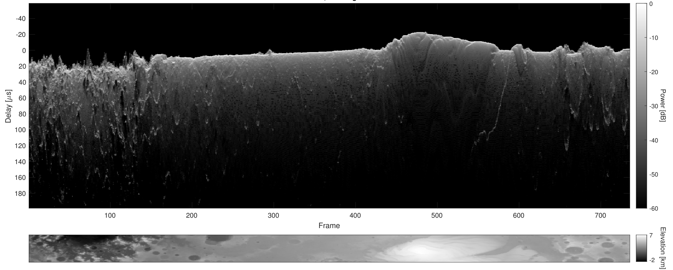
Orbit 6612, Cluttergram
