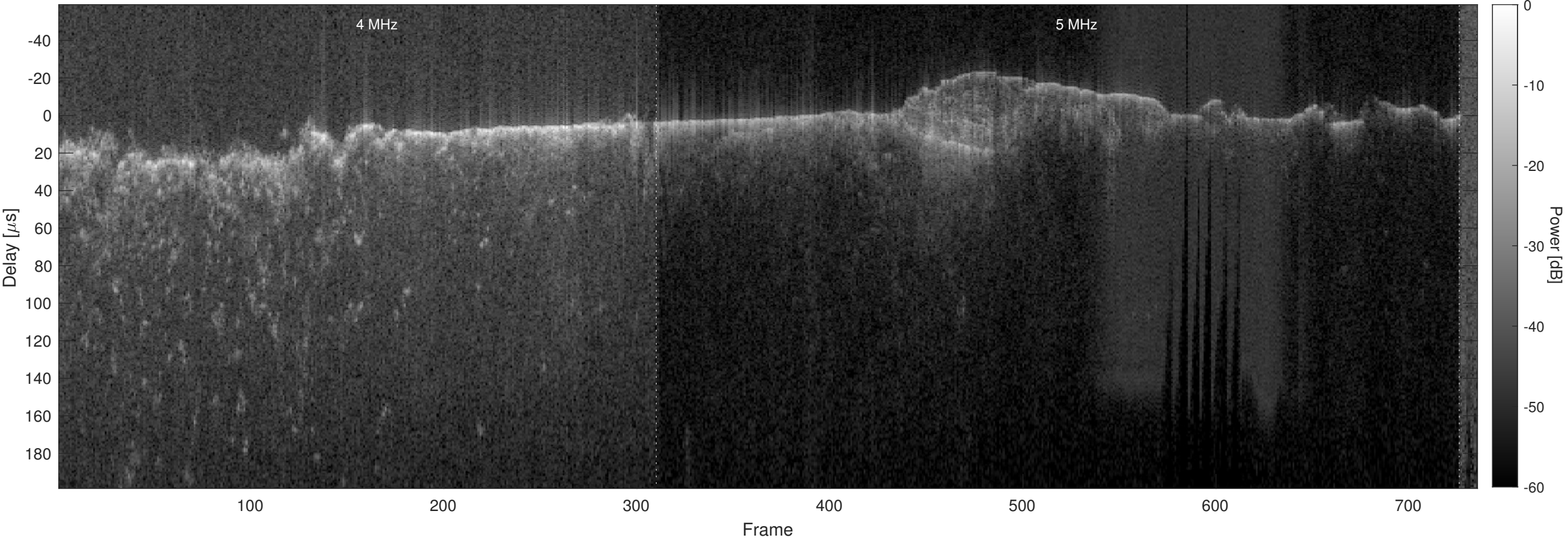
Orbit 6612, Optimized, No Window, Channel 2
