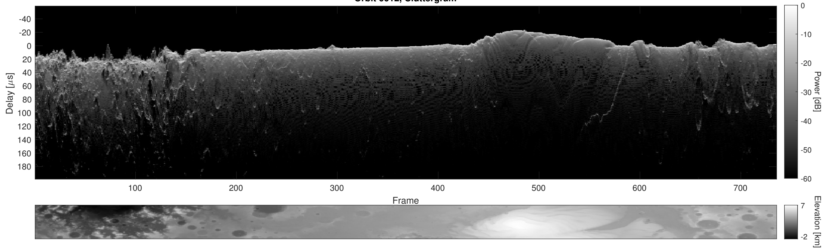
Orbit 6612, Cluttergram
