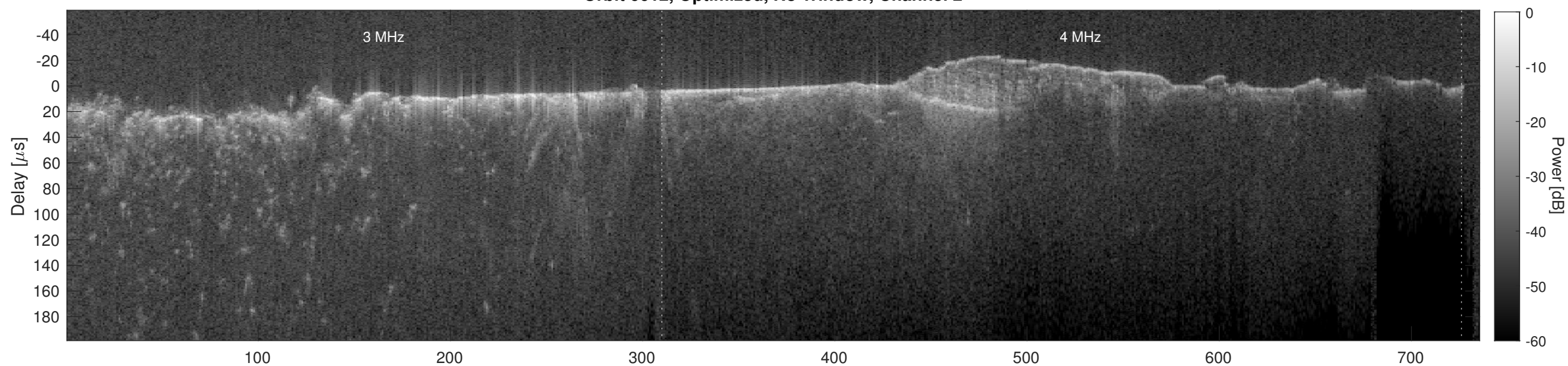
Orbit 6612, Cluttergram
