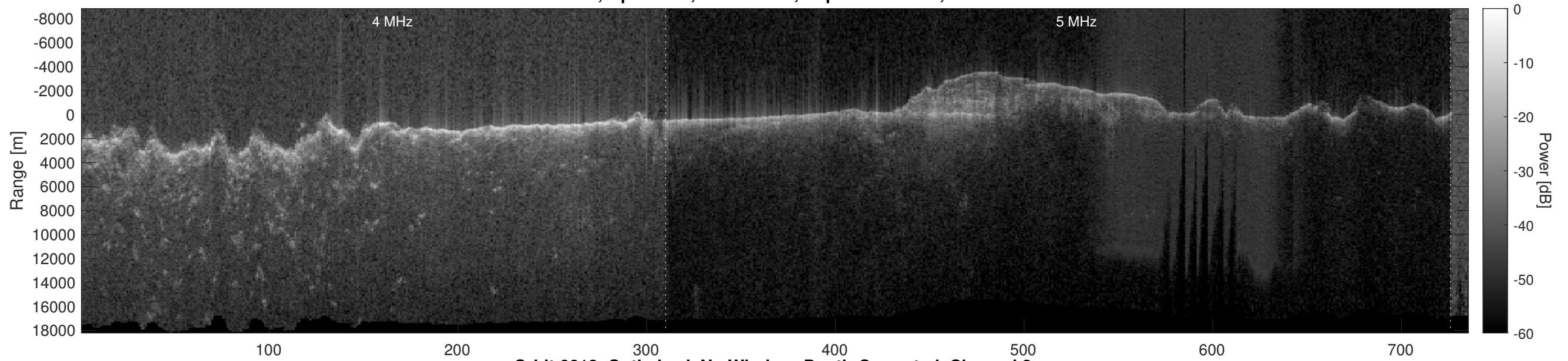
Orbit 6612, Optimized, No Window, Depth-Corrected, Channel 2
