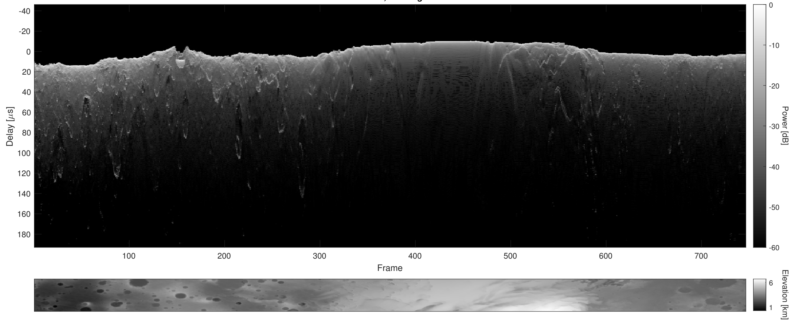
Orbit 6617, Cluttergram
