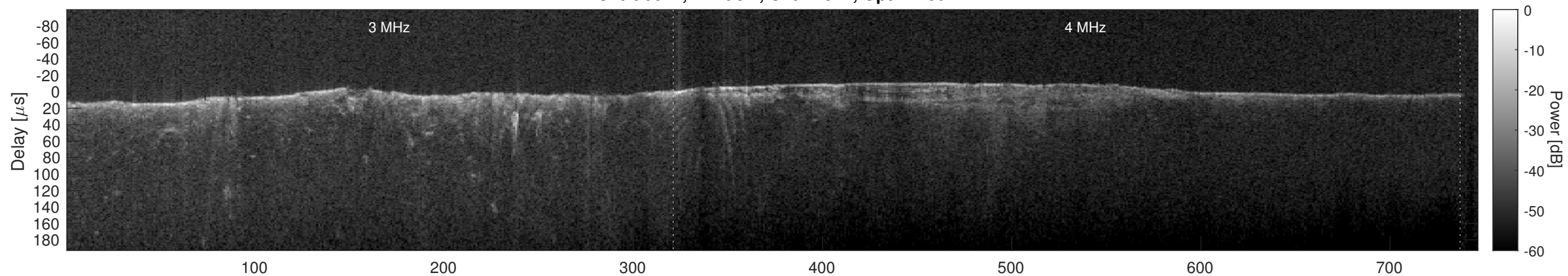
Orbit 6617, Cluttergram
