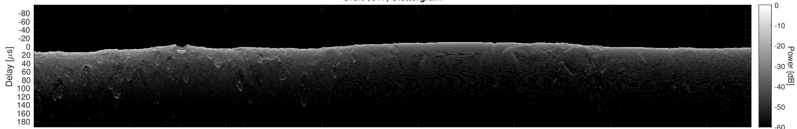
Orbit 6617, Cluttergram
