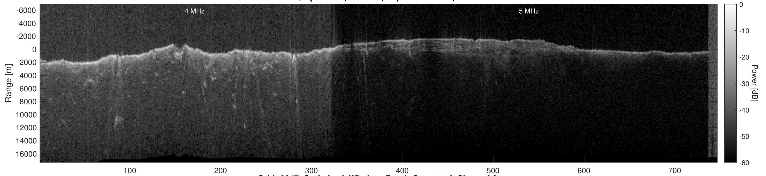
Orbit 6617, Optimized, Window, Depth-Corrected, Channel 2
