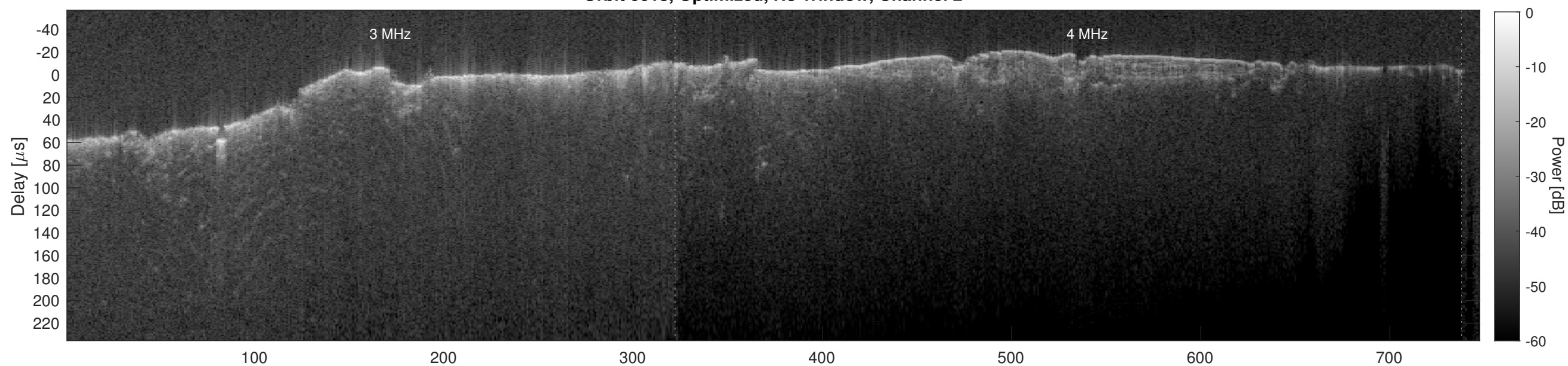
Orbit 6618, Cluttergram
