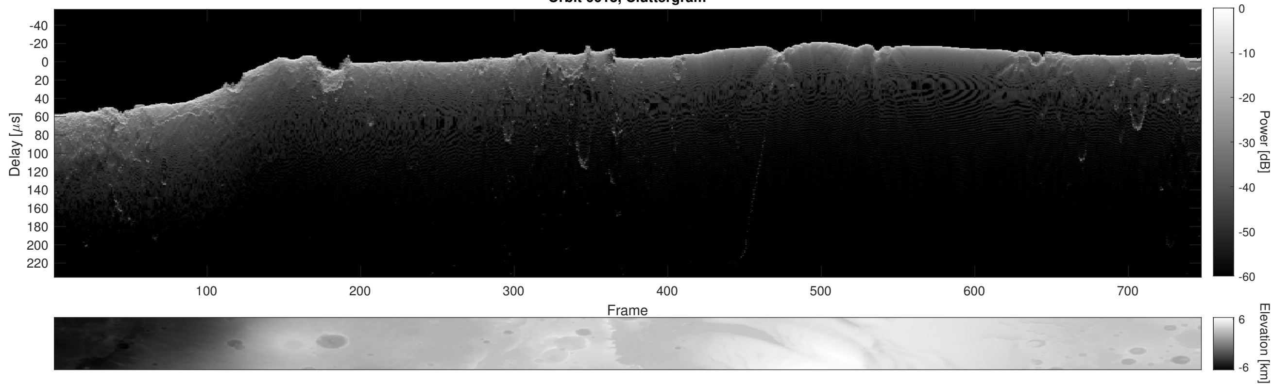
Orbit 6618, Cluttergram
