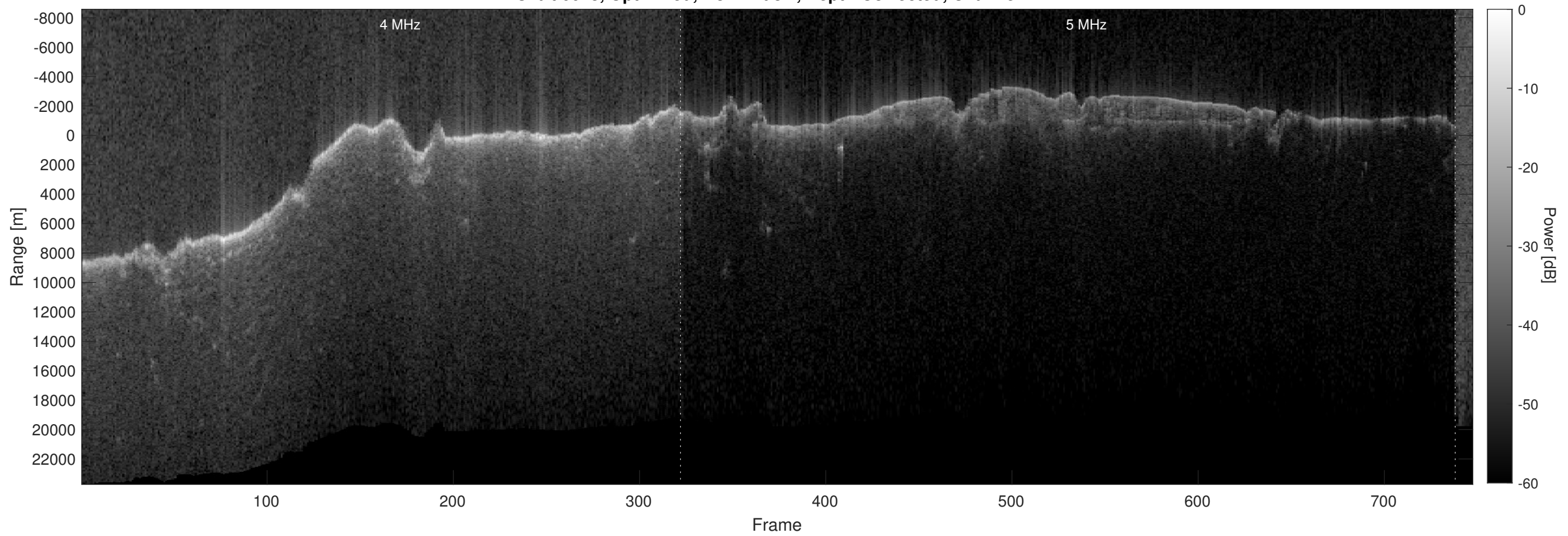
Orbit 6618, Optimized, No Window, Depth-Corrected, Channel 2
