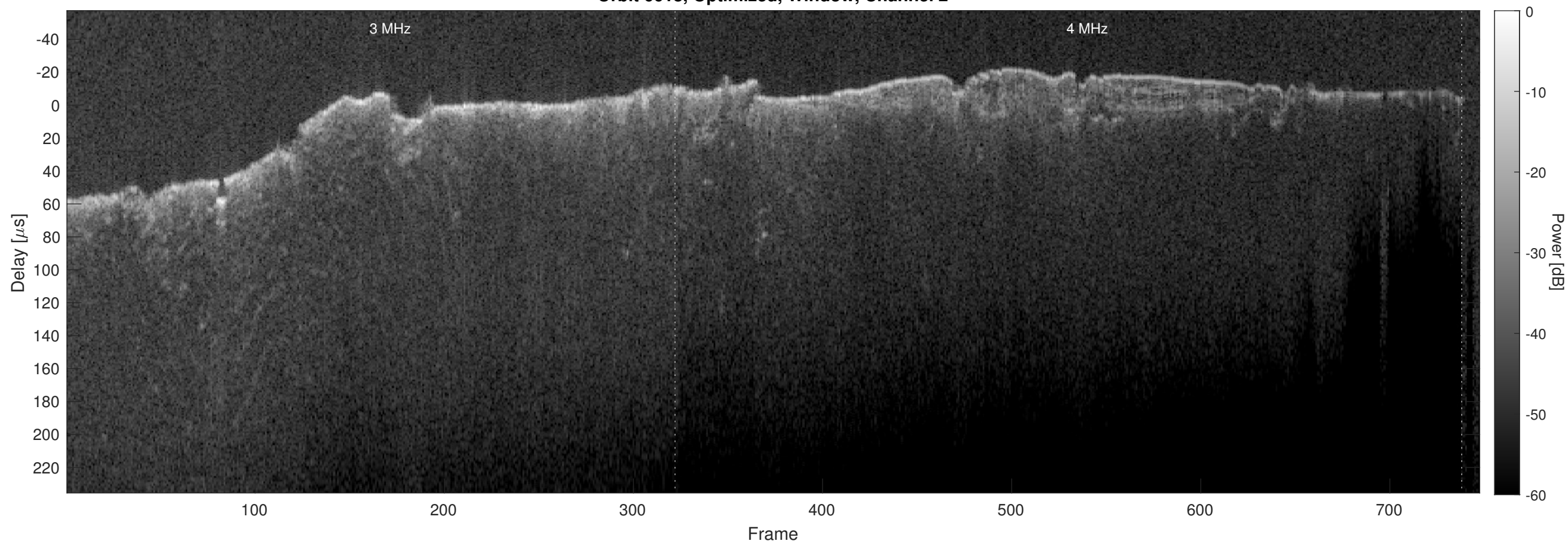
Orbit 6618, Optimized, Window, Channel 2
