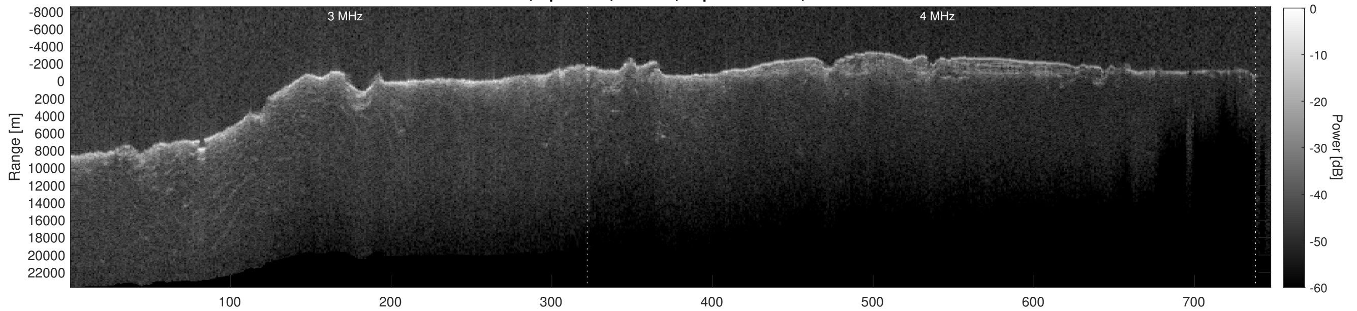
Orbit 6618, Depth-Corrected Cluttergram
