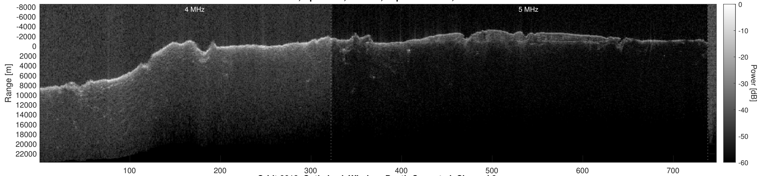
Orbit 6618, Optimized, Window, Depth-Corrected, Channel 2
