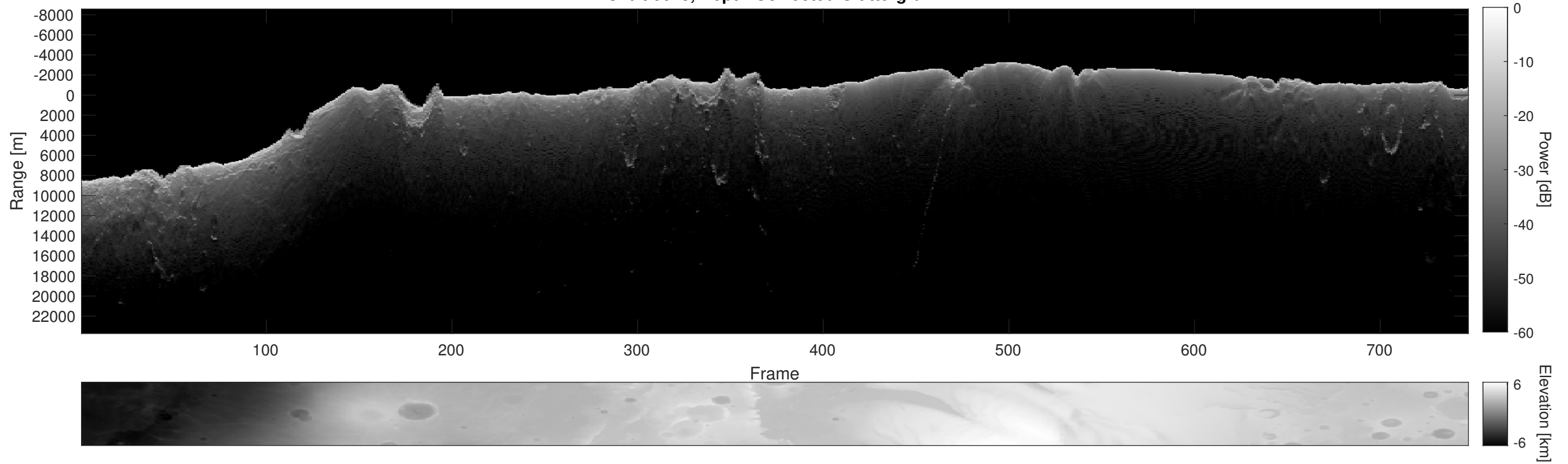
Orbit 6618, Depth-Corrected Cluttergram
