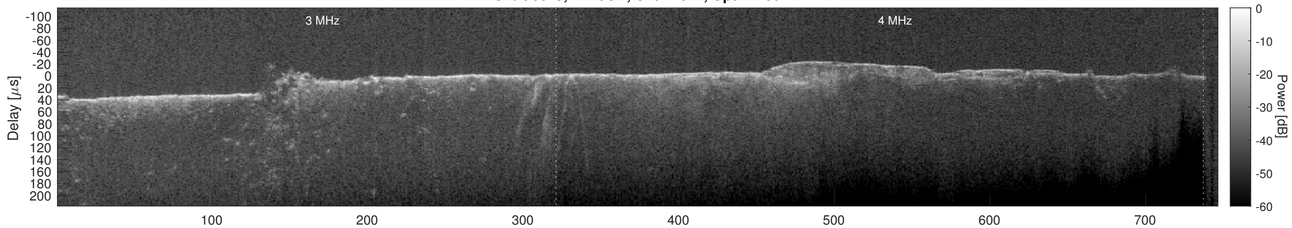
Orbit 6619, Cluttergram
