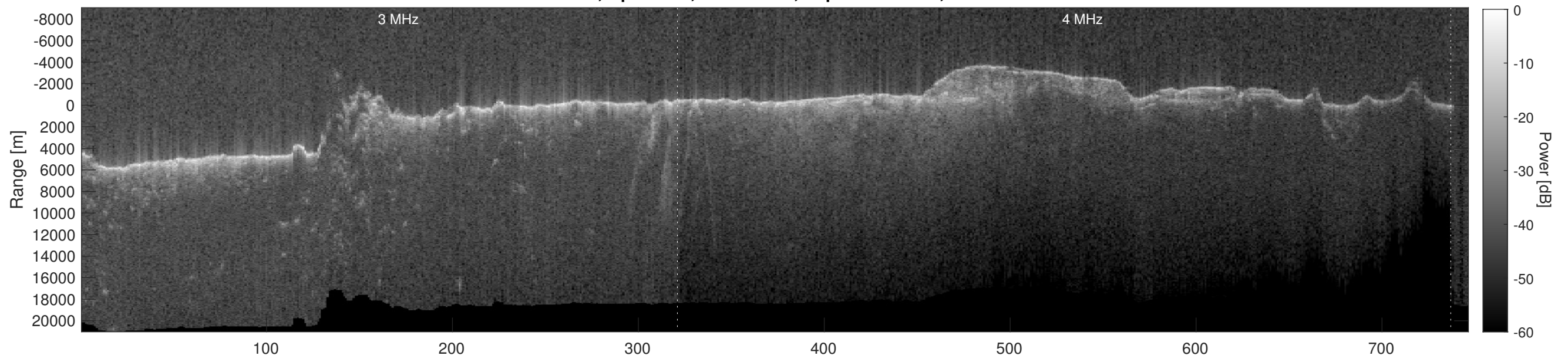
Orbit 6619, Depth-Corrected Cluttergram
