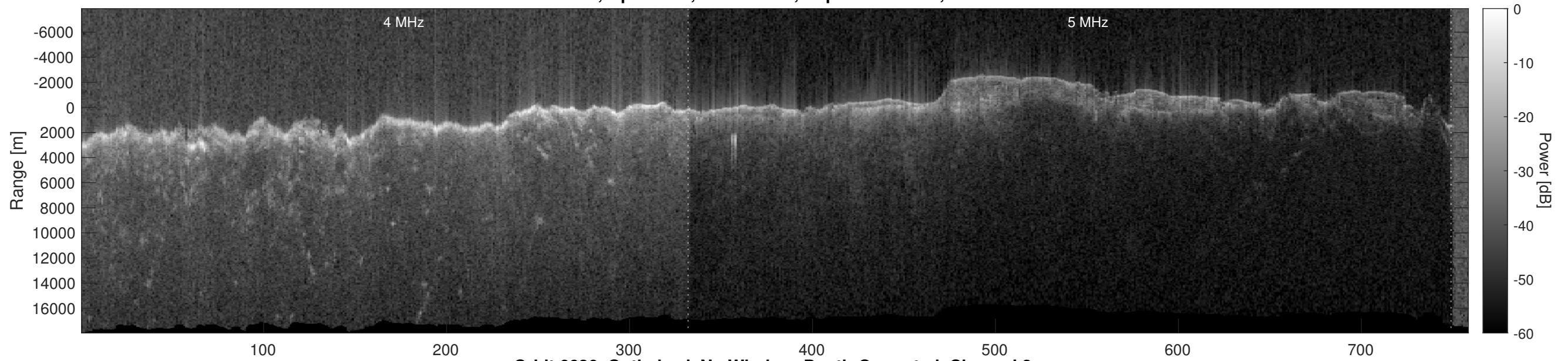
Orbit 6626, Optimized, No Window, Depth-Corrected, Channel 2
