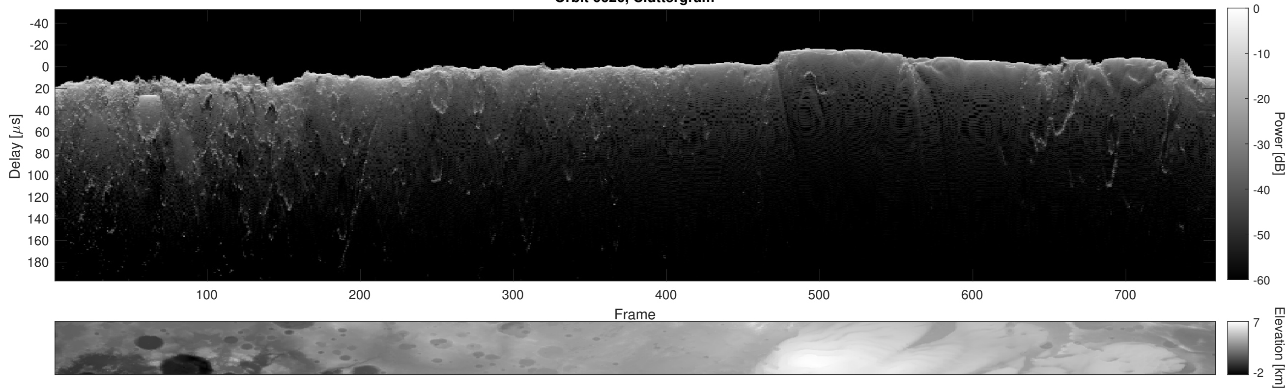
Orbit 6626, Cluttergram
