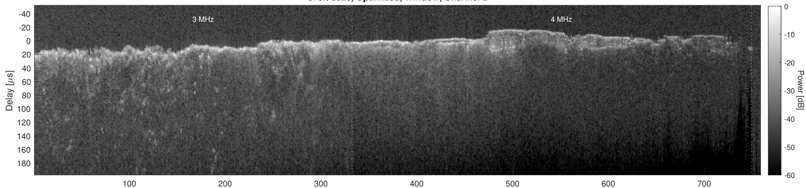
Orbit 6626, Cluttergram
