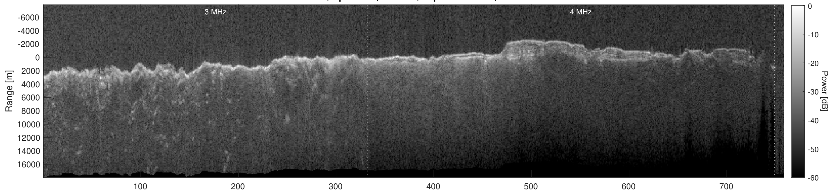
Orbit 6626, Depth-Corrected Cluttergram
