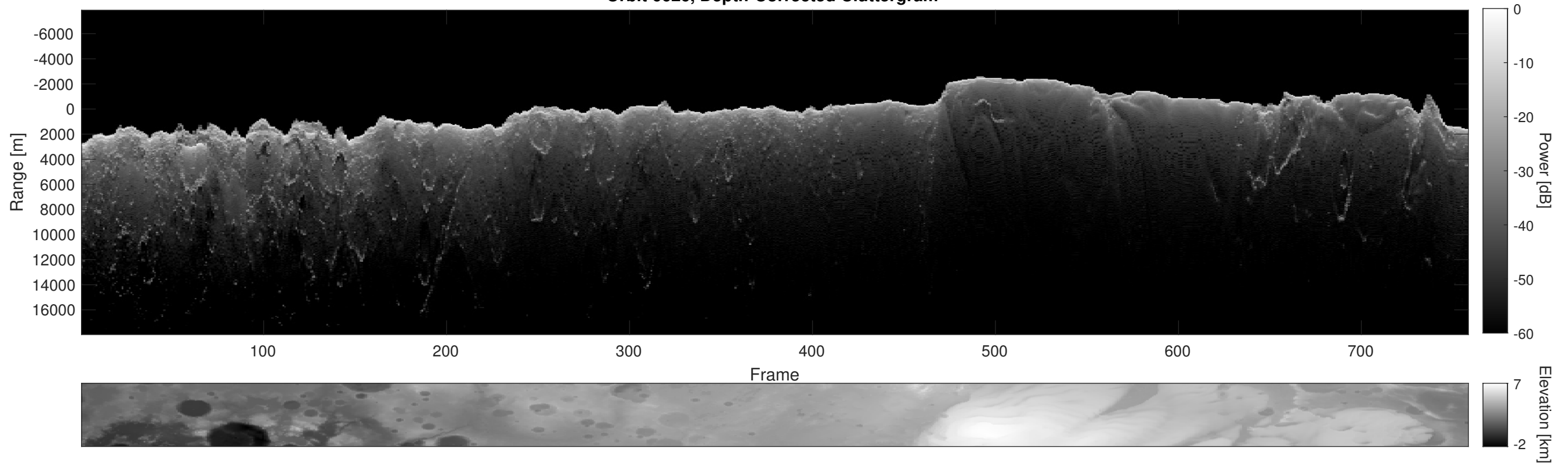
Orbit 6626, Depth-Corrected Cluttergram
