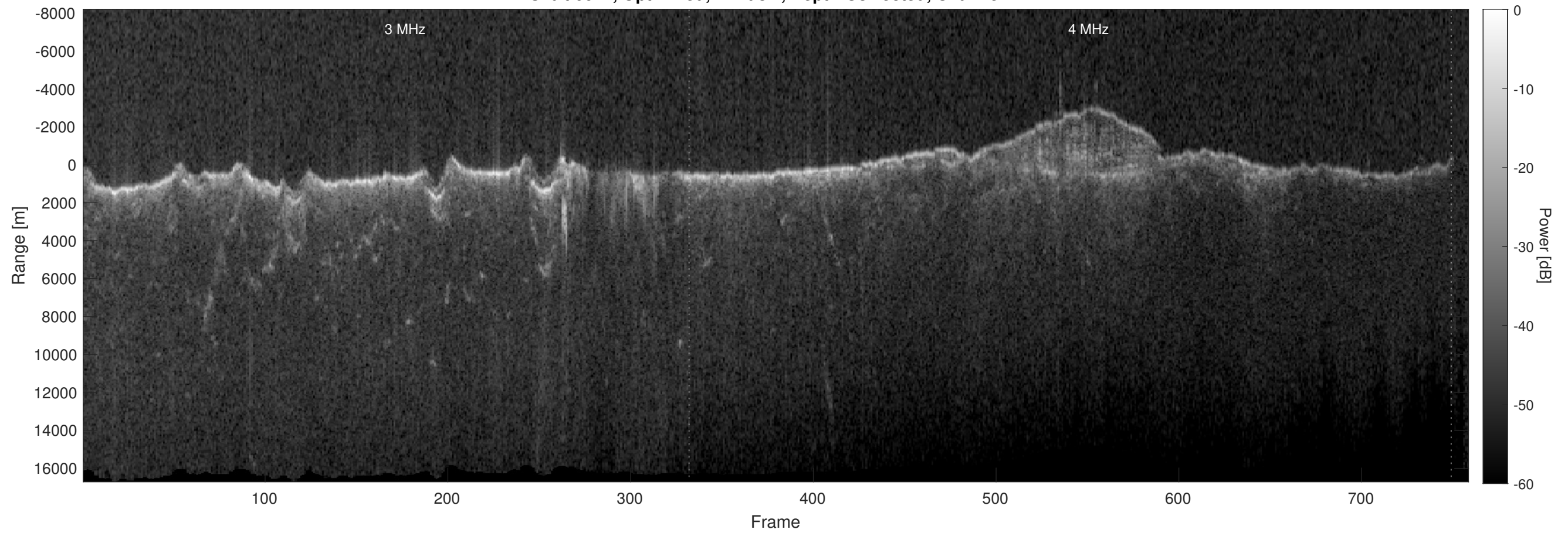
Orbit 6627, Optimized, Window, Depth-Corrected, Channel 2
