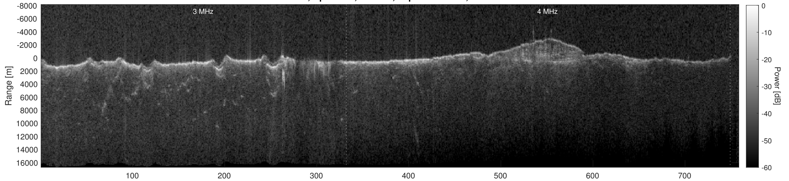
Orbit 6627, Depth-Corrected Cluttergram
