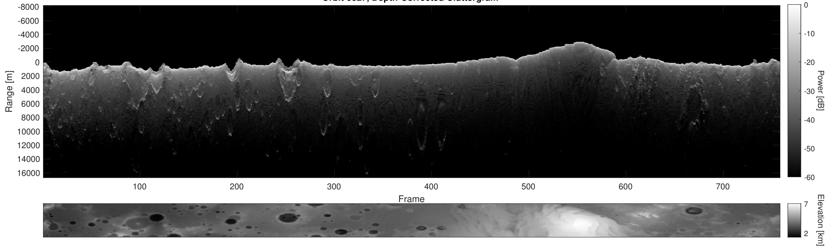
Orbit 6627, Depth-Corrected Cluttergram
