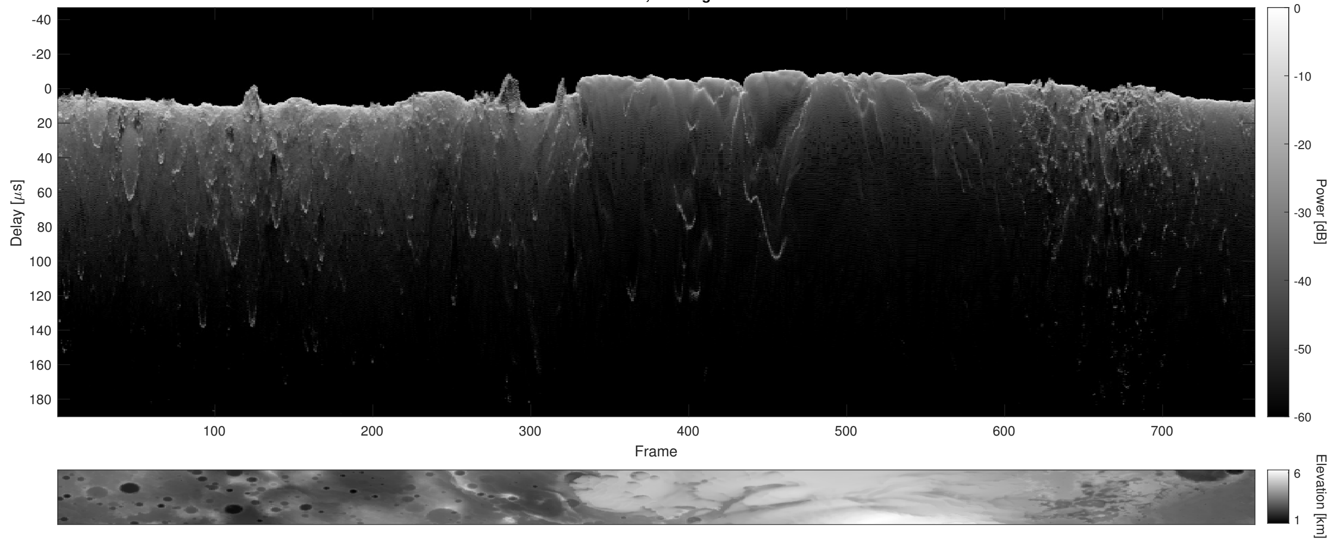
Orbit 6628, Cluttergram
