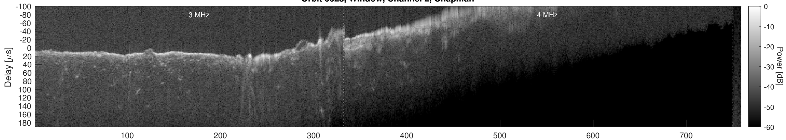
Orbit 6628, Window, Channel 2, Optimized
