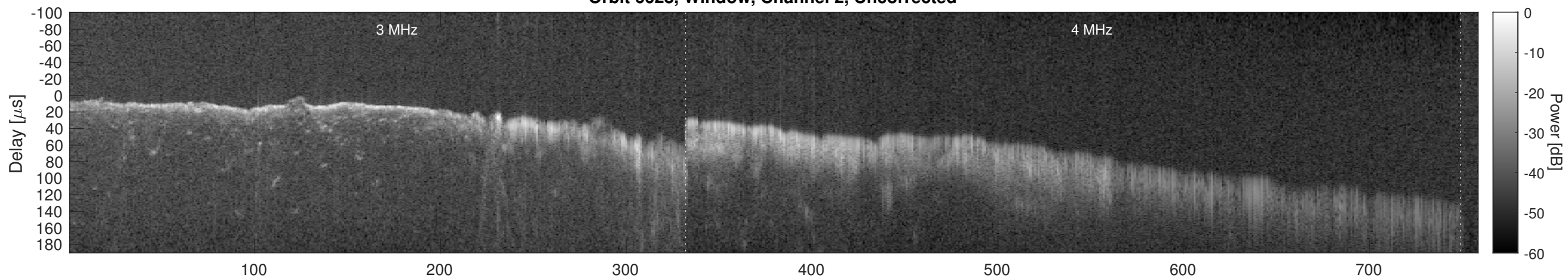
Orbit 6628, Window, Channel 2, Chapman
