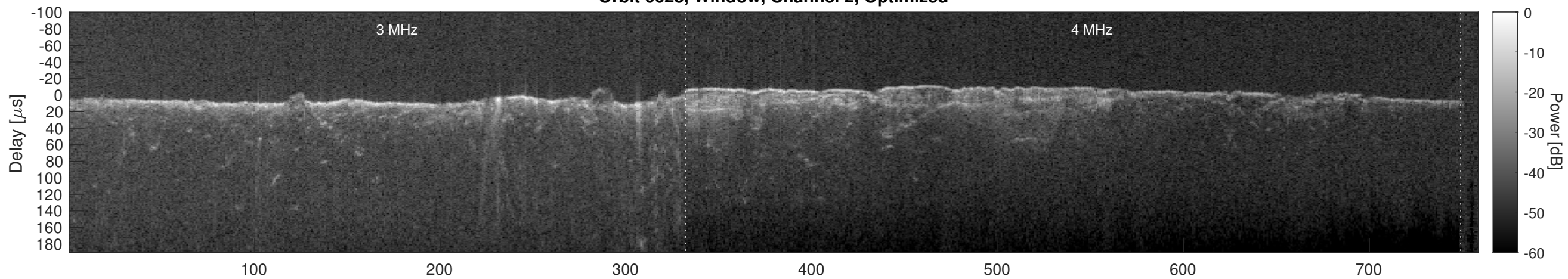
Orbit 6628, Cluttergram
