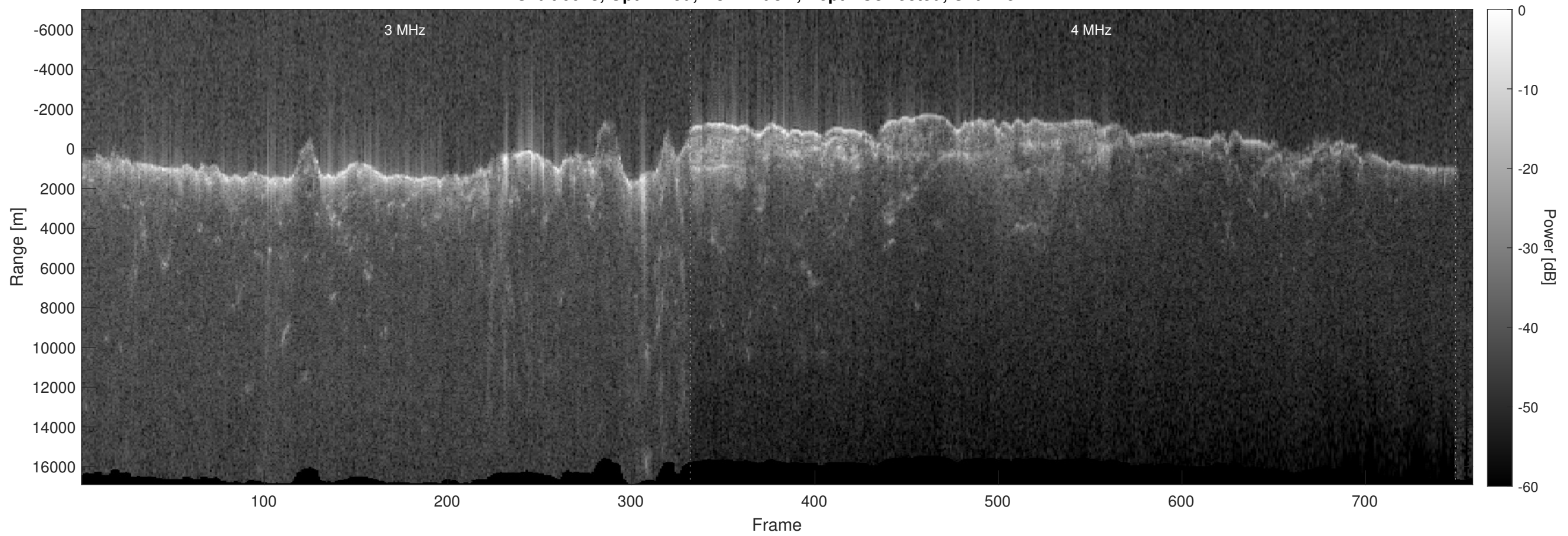
Orbit 6628, Optimized, No Window, Depth-Corrected, Channel 2
