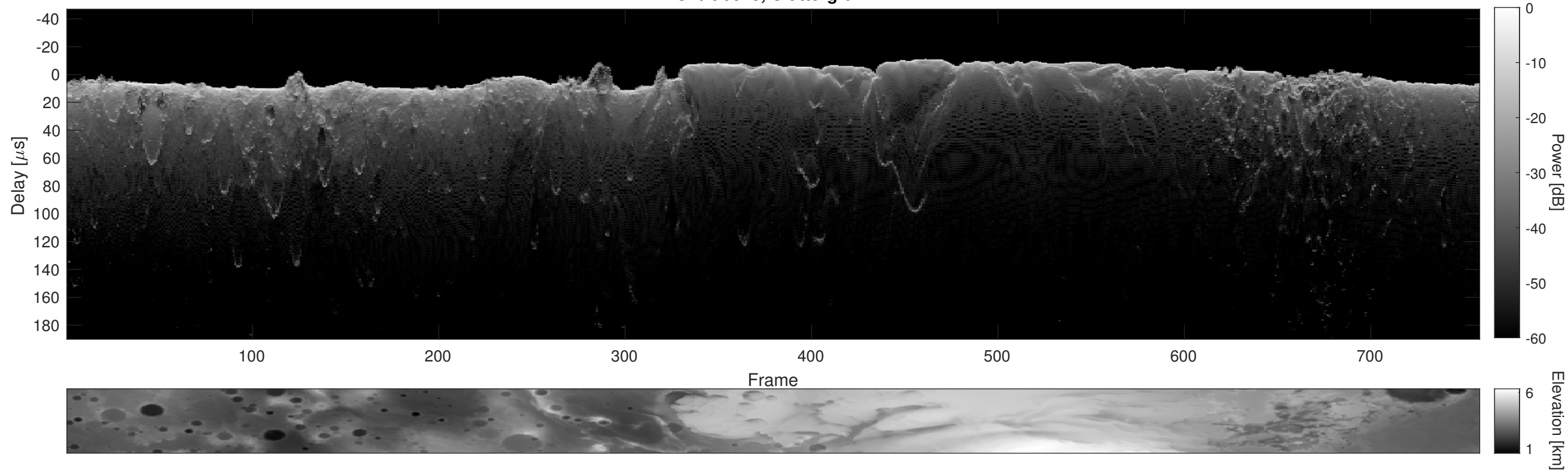
Orbit 6628, Cluttergram
