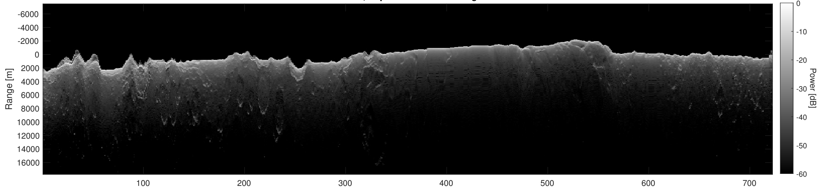
Orbit 6631, Depth-Corrected Cluttergram
