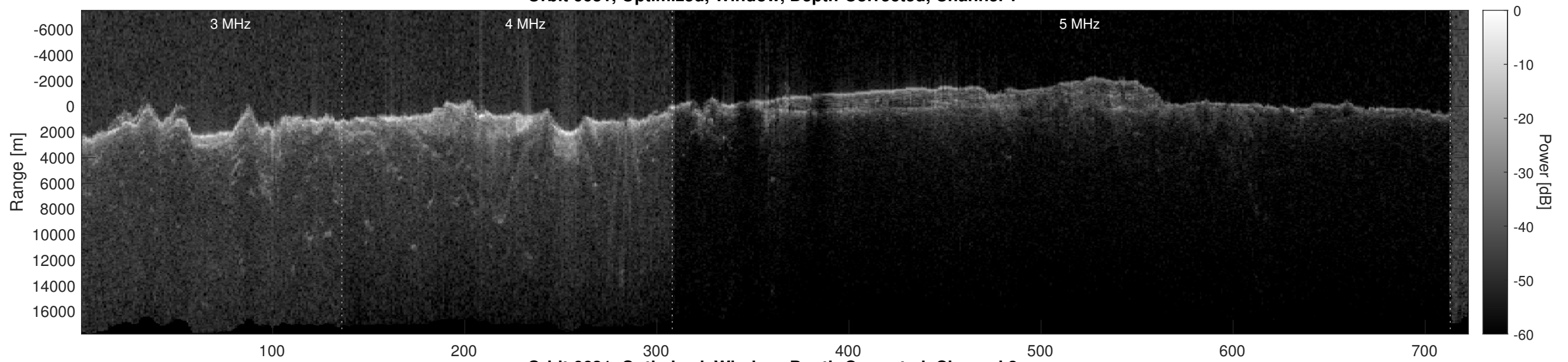
Orbit 6631, Optimized, Window, Depth-Corrected, Channel 2
