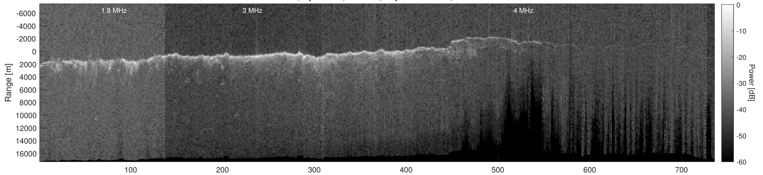
Orbit 6633, Depth-Corrected Cluttergram
