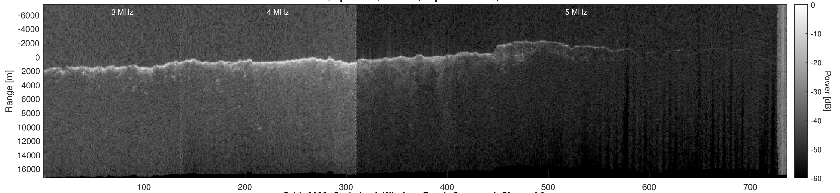
Orbit 6633, Optimized, Window, Depth-Corrected, Channel 2
